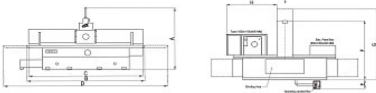
MACHINE LAYOUT
